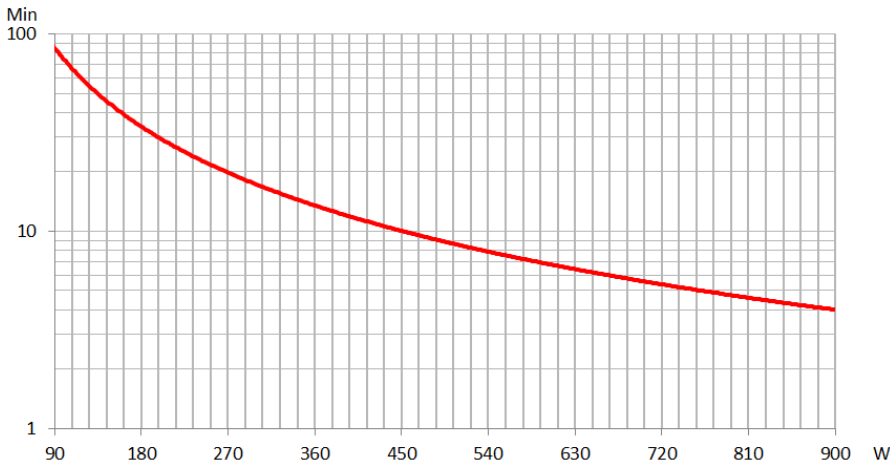
Figure 13 – Runtime graph of SMALLT1A5
