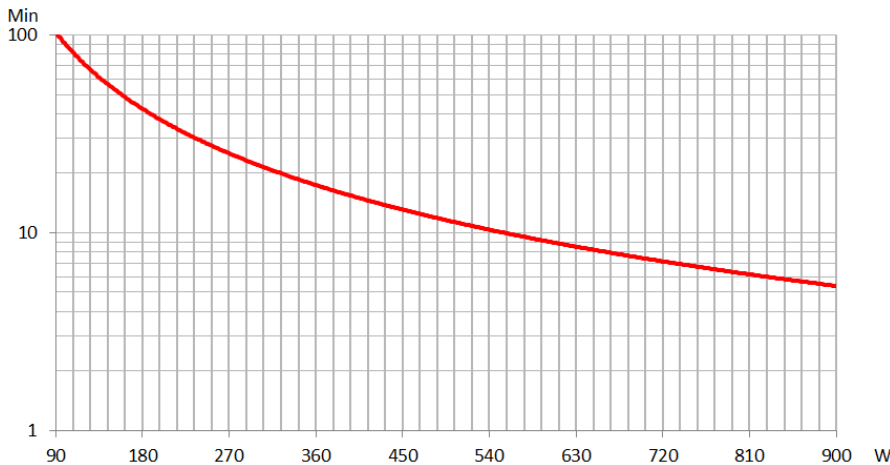
Figure 14 – Runtime graph of SMALLT1A10
