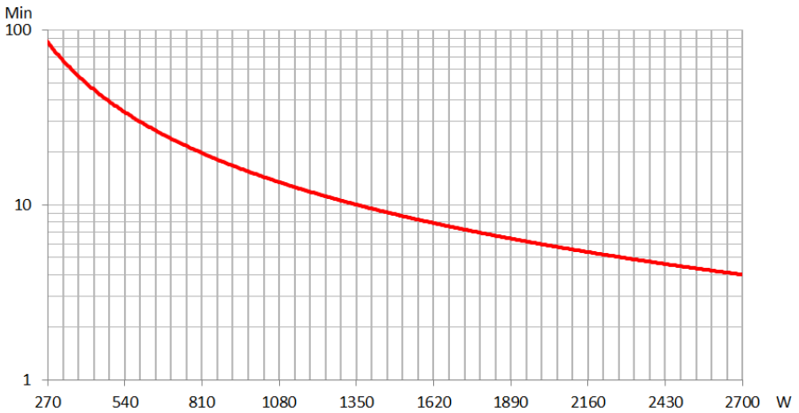
Figure 17 – Runtime graph of SMALLT3A5
