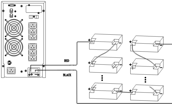
Figure 4 – External batteries connection.
