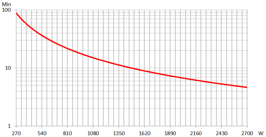
Figure 18 – Runtime graph of SMALLT3A10
