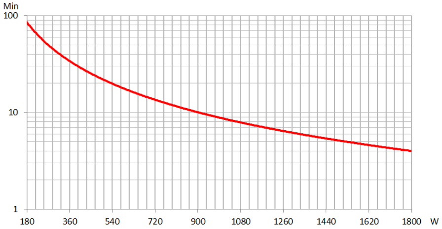
Figure 15 – Runtime graph of SMALLT2A5
