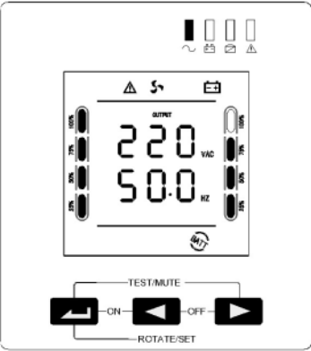
Figure 8 - Screen with UPS control buttons
